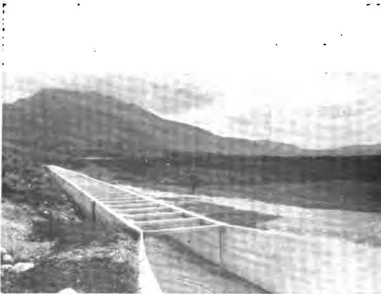
FIG. 146.—Concrete Flume, Spanish Fork Valley, Utah, showing Warped Transition from Canal to Flume.
